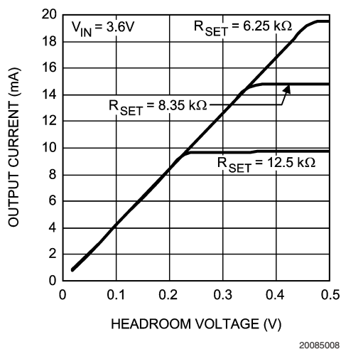
FIGURE 4. I_{LED} vs V_{HR} 3 LEDs, V_{IN} = 3.6V
